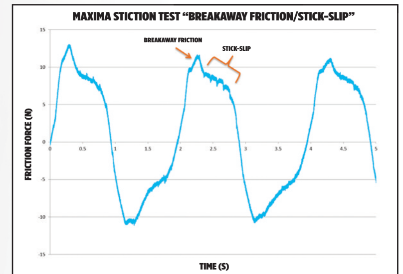
STICTION TEST BREAKAWAY FRICTION / STICK SLIP
